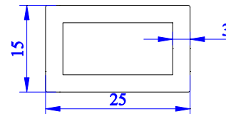
4896 - 0.551 kg/m
