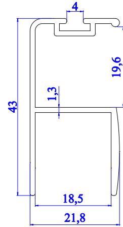
4862 - 0.410 kg/m
